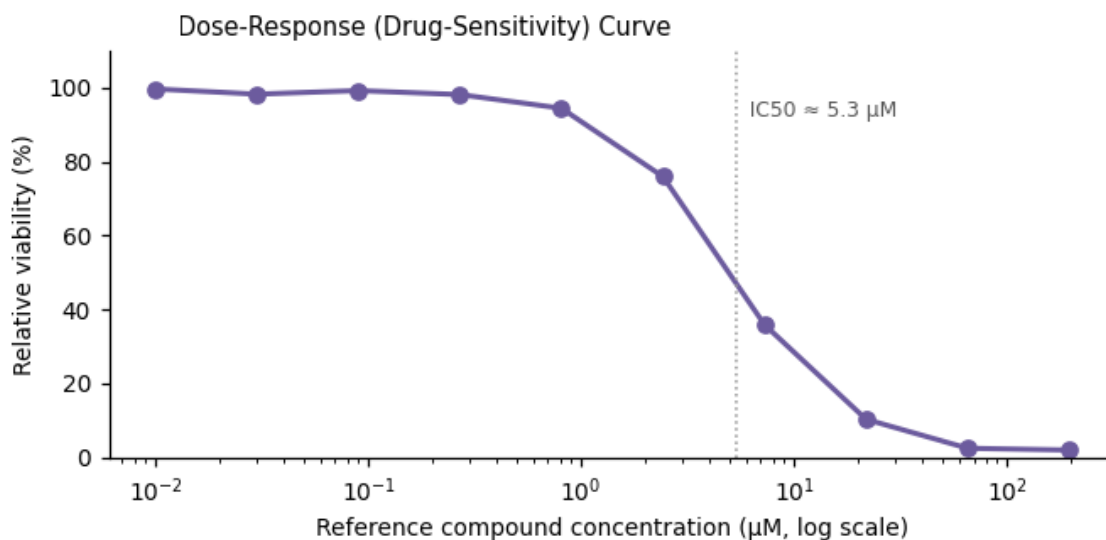
Figure 3. Functional assay readout — \text{IC}_{50} \approx 5.3 \mu\text{M} .
