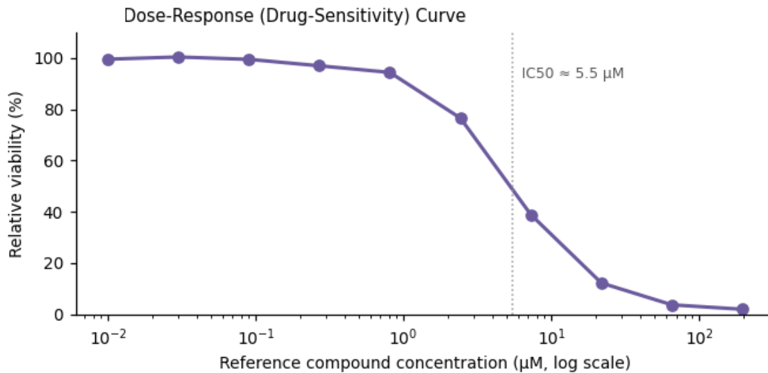
Figure 3. Functional assay readout — IC 50 ≈ 5.5 μM.
