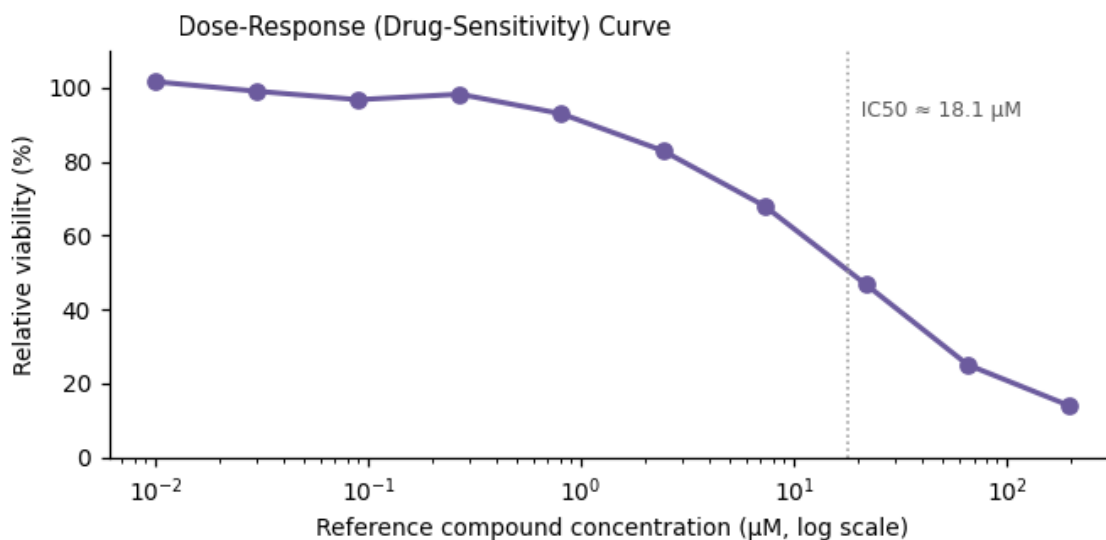
Figure 3. Functional assay readout — \text{IC}_{50} \approx 18.1 \mu\text{M} .
