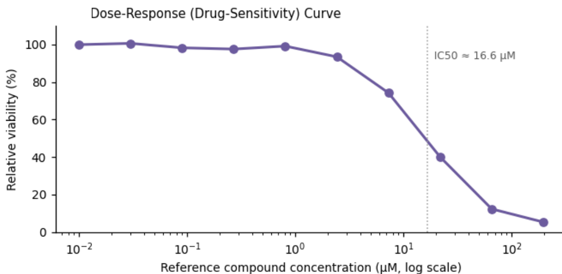
Figure 3. Functional assay readout — IC 50 ≈ 16.6 μM.
