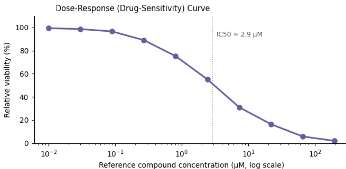
Figure 3. Functional assay readout — \text{IC}_{50} \approx 2.9 \mu\text{M} .
