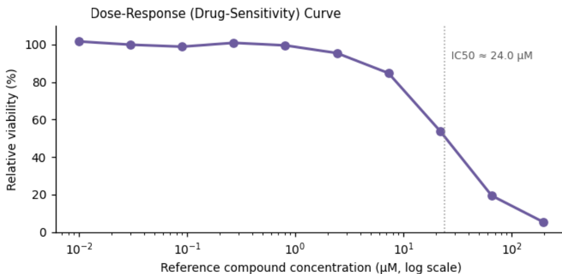
Figure 3. Functional assay readout — IC 50 ≈ 24.0 μM.
