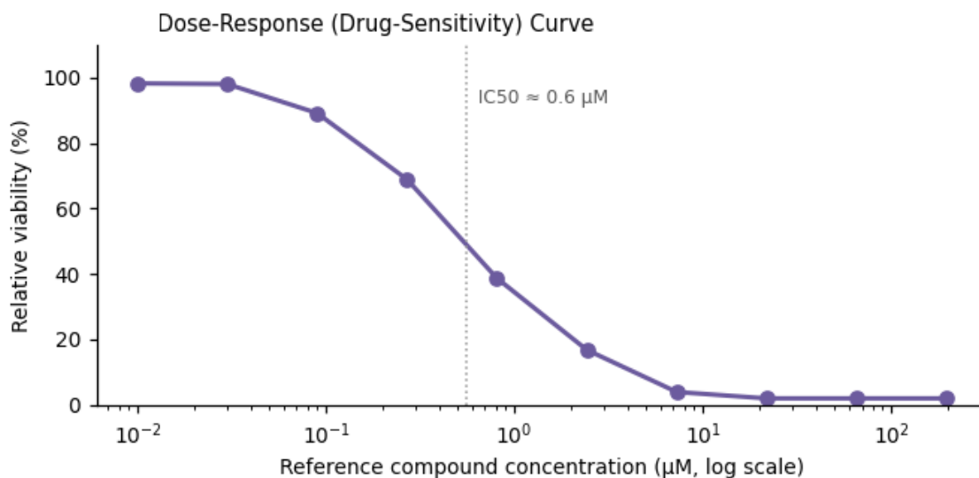
Figure 3. Functional assay readout — IC 50 ≈ 0.6 μM.
