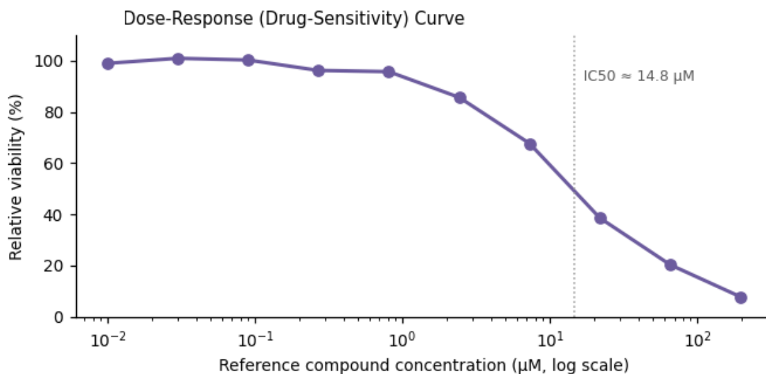
Figure 3. Functional assay readout — IC 50 ≈ 14.8 μM.
