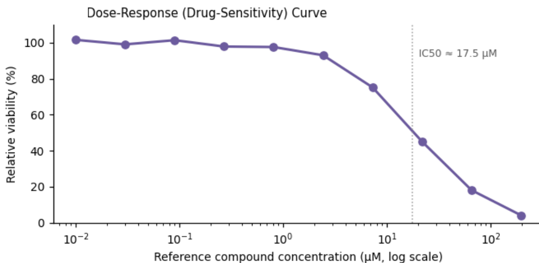
Figure 3. Functional assay readout — IC 50 ≈ 17.5 μM.
