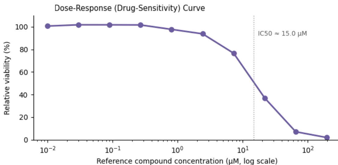
Figure 3. Functional assay readout — IC 50 ≈ 15.0 μM.
