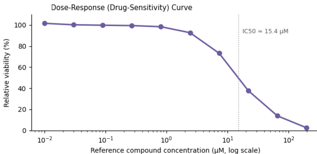
Figure 3. Functional assay readout — IC 50 ≈ 15.4 μM.
