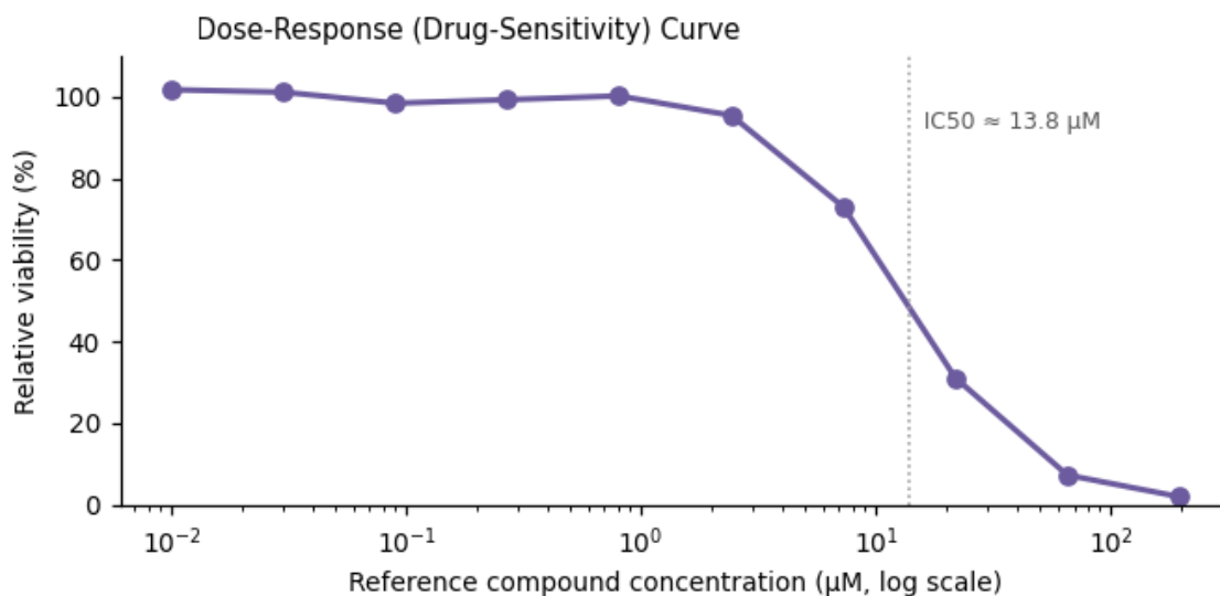
Figure 3. Functional assay readout — IC 50 ≈ 13.8 μM.
