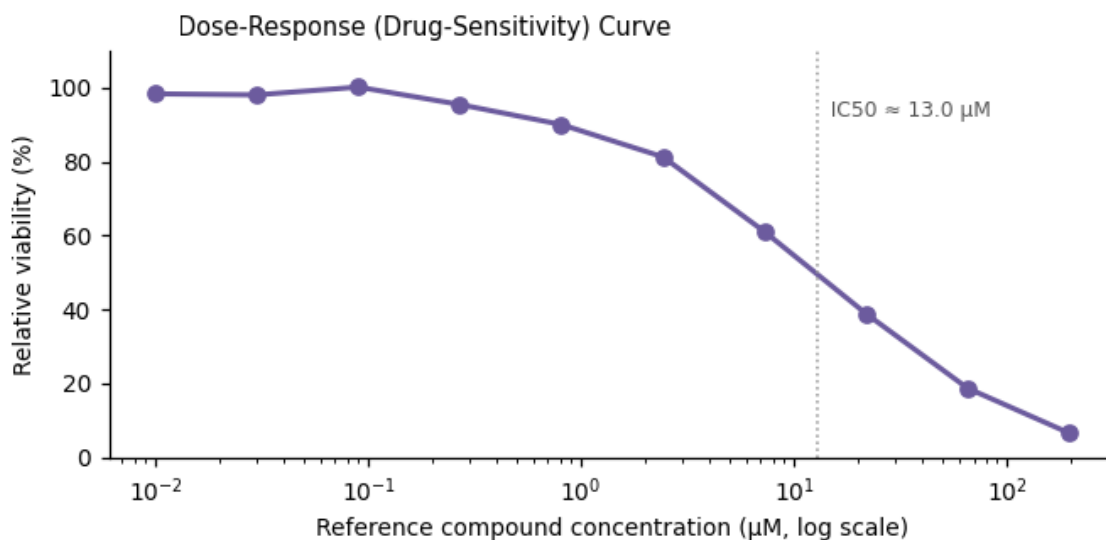
Figure 3. Functional assay readout — \text{IC}_{50} \approx 13.0 \mu\text{M} .
