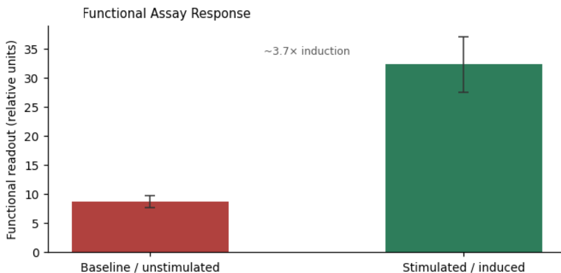
Figure 3. Functional assay readout — \sim 3.7\times induction over baseline.
