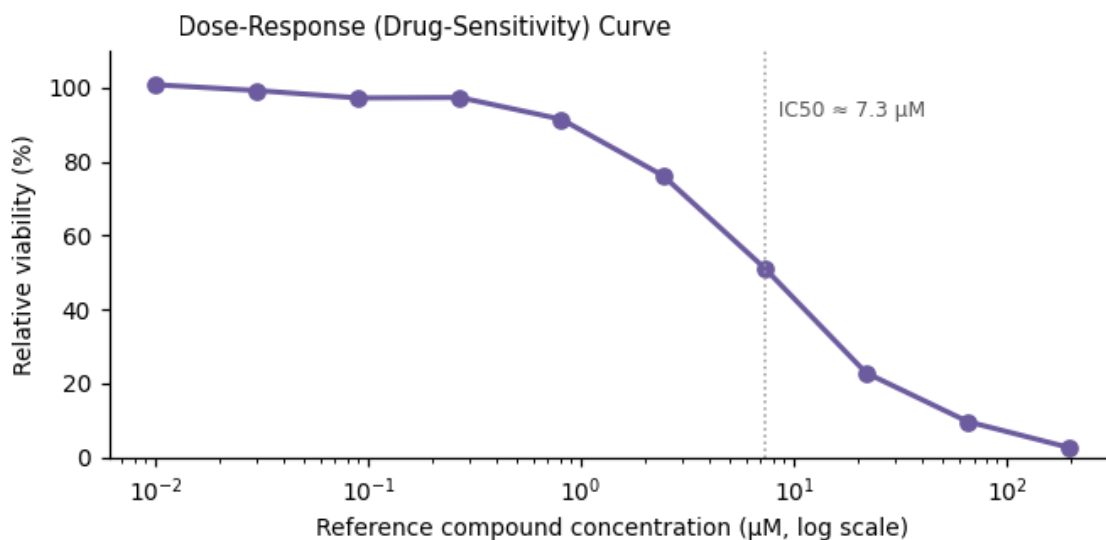
Figure 3. Functional assay readout — \text{IC}_{50} \approx 7.3 \mu\text{M} .
