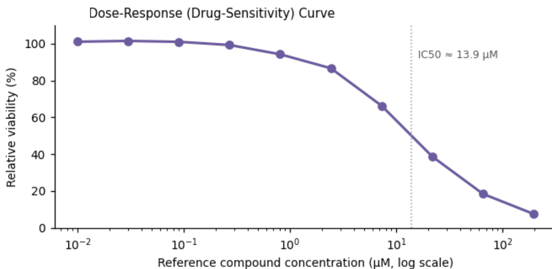
Figure 3. Functional assay readout — IC 50 ≈ 13.9 μM.
