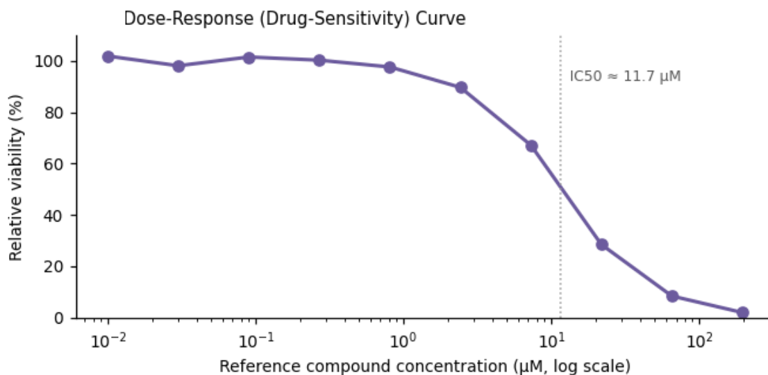
Figure 3. Functional assay readout — IC 50 ≈ 11.7 μM.
