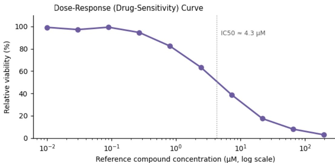
Figure 3. Functional assay readout — \text{IC}_{50} \approx 4.3 \mu\text{M} .
