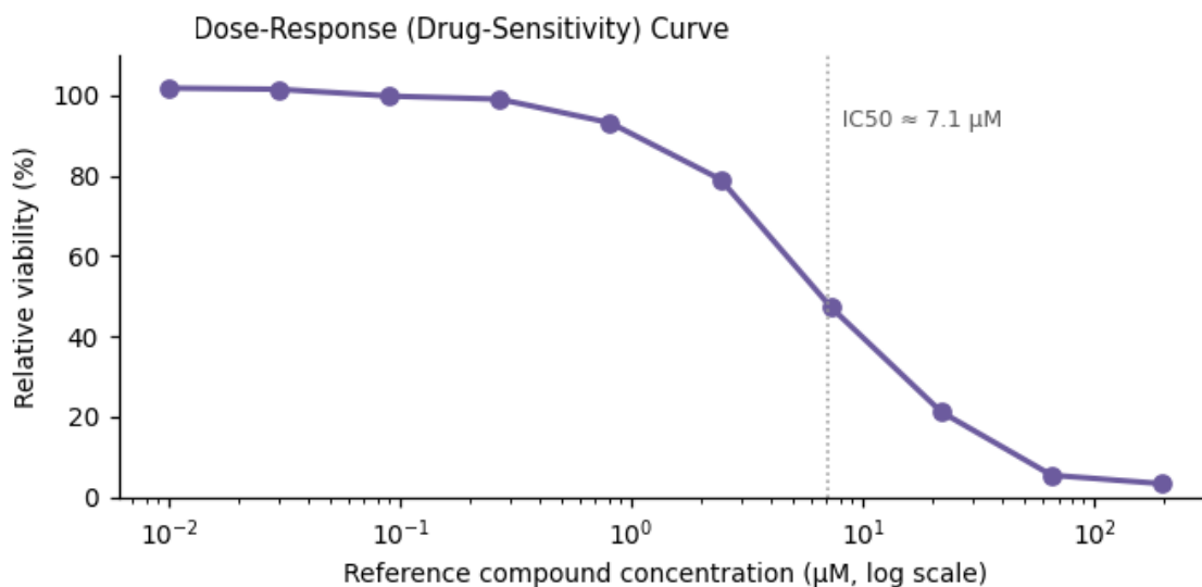
Figure 3. Functional assay readout — IC 50 ≈ 7.1 µM.
