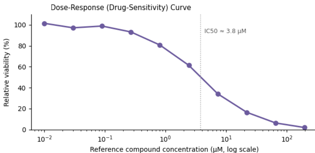
Figure 3. Functional assay readout — \text{IC}_{50} \approx 3.8 \mu\text{M} .
