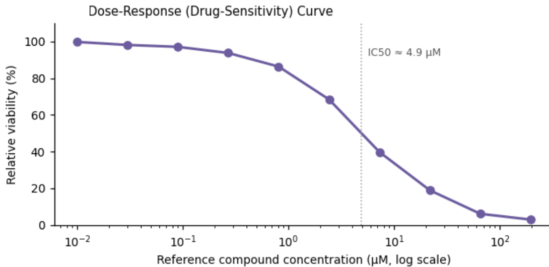
Figure 3. Functional assay readout — \text{IC}_{50} \approx 4.9 \mu\text{M} .
