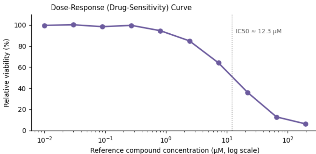
Figure 3. Functional assay readout — IC 50 ≈ 12.3 μM.
