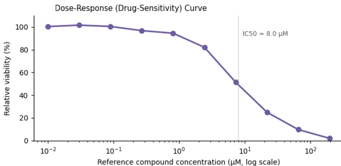
Figure 3. Functional assay readout — IC 50 ≈ 8.0 μM.
