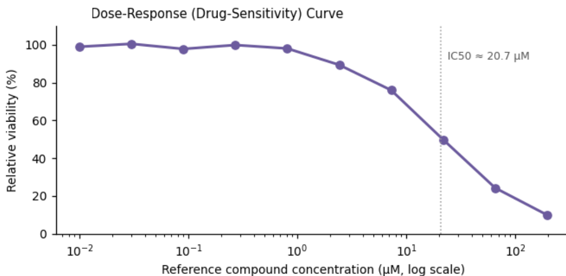
Figure 3. Functional assay readout — IC 50 ≈ 20.7 μM.
