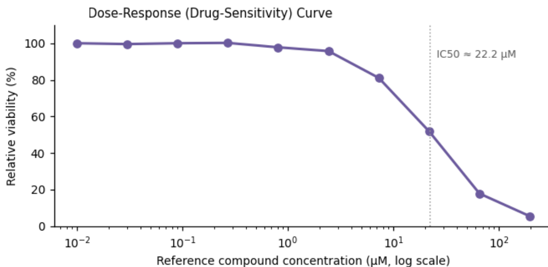
Figure 3. Functional assay readout — IC 50 ≈ 22.2 μM.
