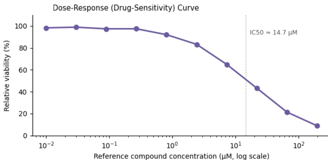
Figure 3. Functional assay readout — \text{IC}_{50} \approx 14.7 \mu\text{M} .
