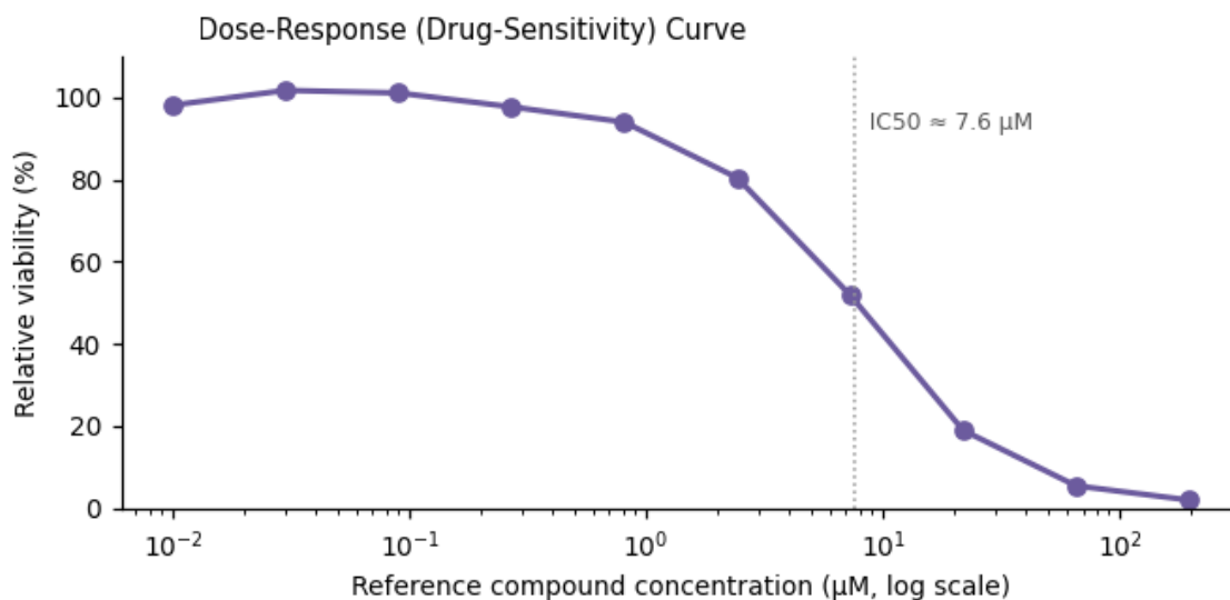
Figure 3. Functional assay readout — \text{IC}_{50} \approx 7.6 \mu\text{M} .
