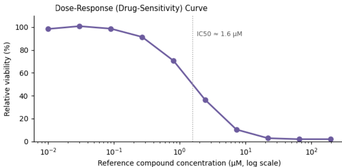
Figure 3. Functional assay readout — IC 50 ≈ 1.6 μM.
