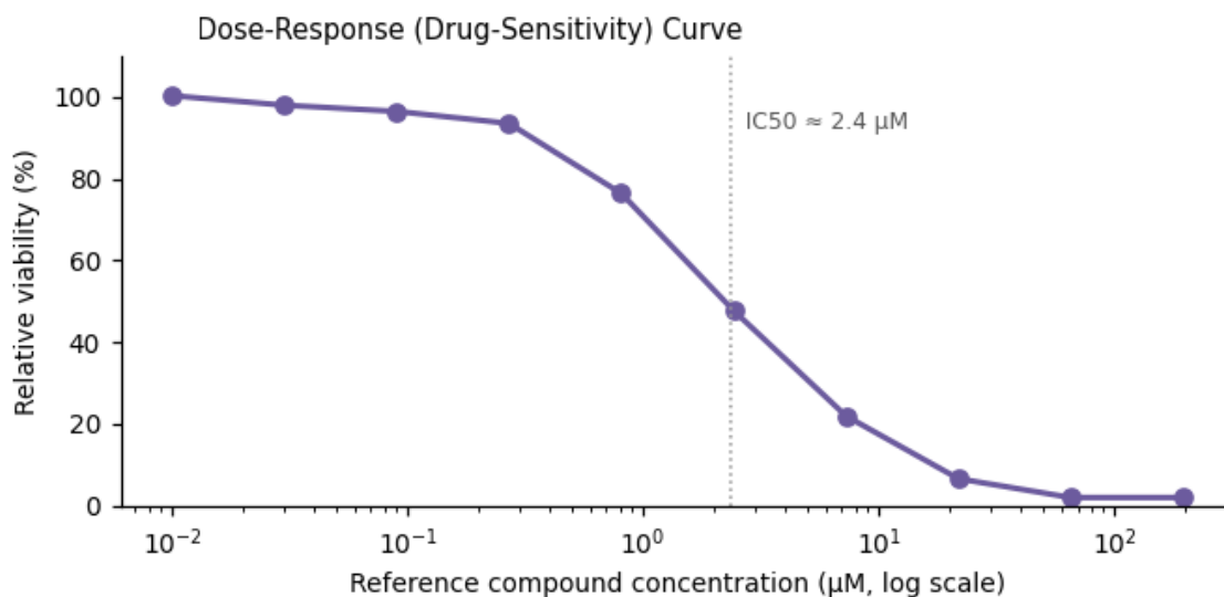
Figure 3. Functional assay readout — \text{IC}_{50} \approx 2.4 \mu\text{M} .
