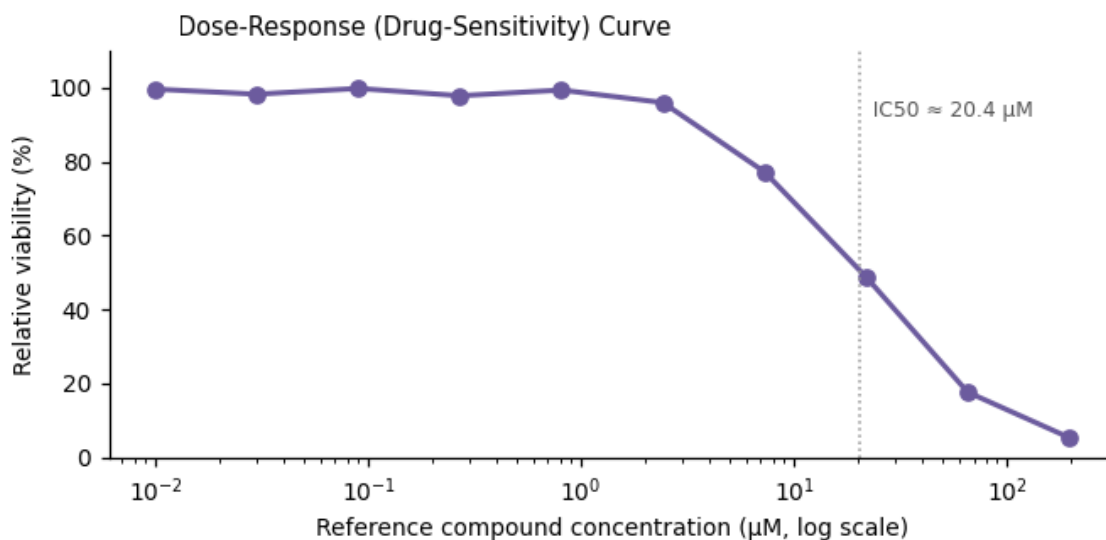
Figure 3. Functional assay readout — IC 50 ≈ 20.4 μM.
