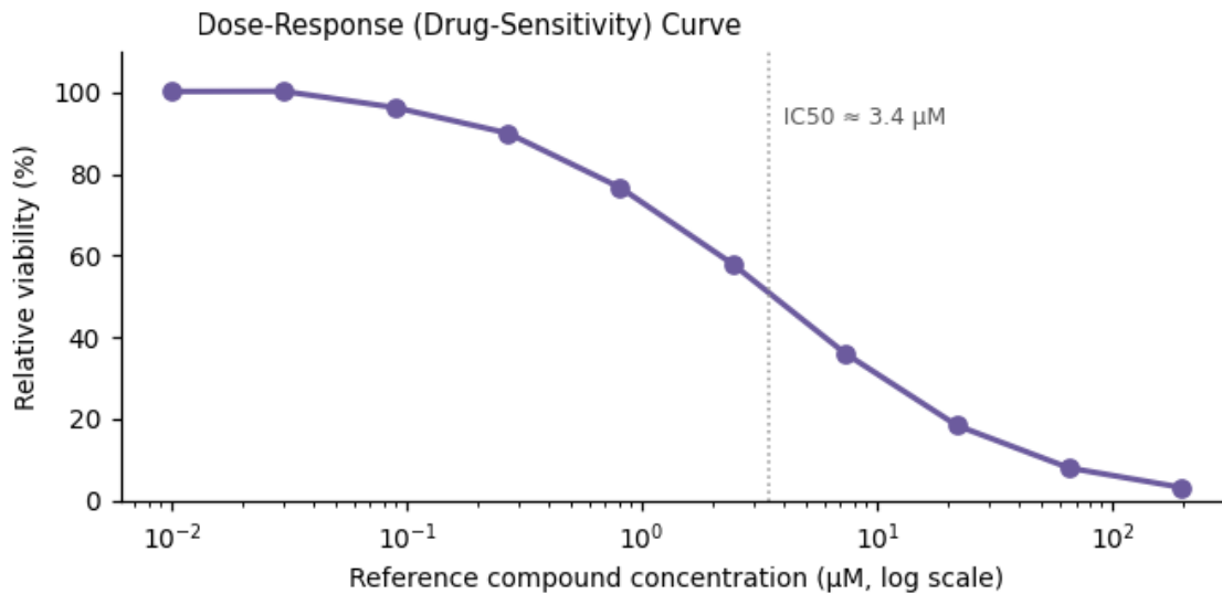
Figure 3. Functional assay readout — \text{IC}_{50} \approx 3.4 \mu\text{M} .
