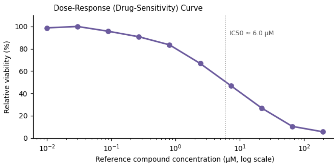
Figure 3. Functional assay readout — \text{IC}_{50} \approx 6.0 \mu\text{M} .
