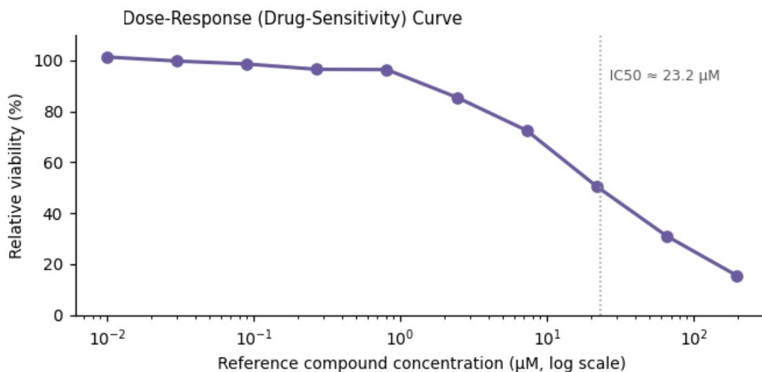
Figure 3. Functional assay readout — \text{IC}_{50} \approx 23.2 \mu\text{M} .
