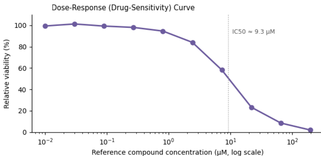
Figure 3. Functional assay readout — \text{IC}_{50} \approx 9.3 \mu\text{M} .
