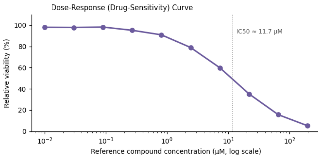
Figure 3. Functional assay readout — \text{IC}_{50} \approx 11.7 \mu\text{M} .
