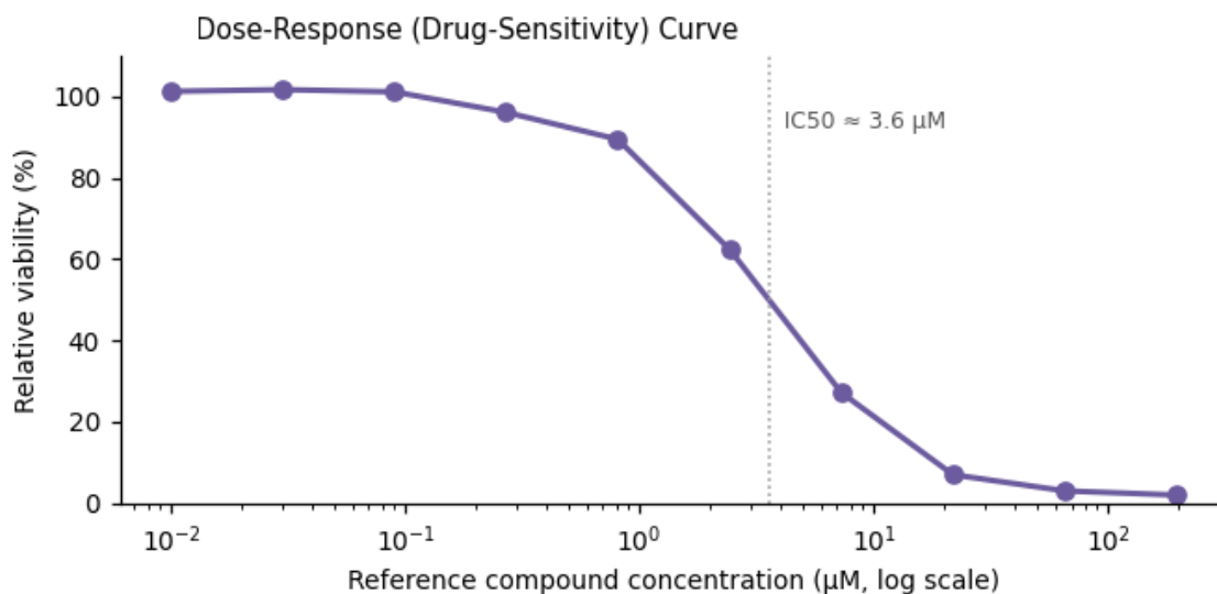
Figure 3. Functional assay readout — IC 50 ≈ 3.6 μM.
